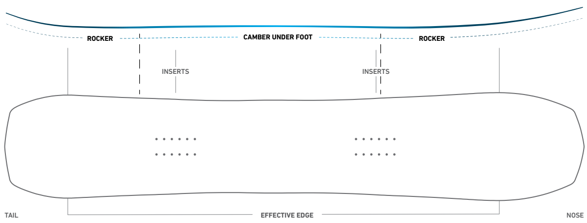
Drawing of the Flagship, size 161
