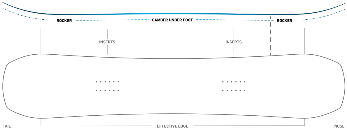
Drawing of the Mountain Twin, size 157
