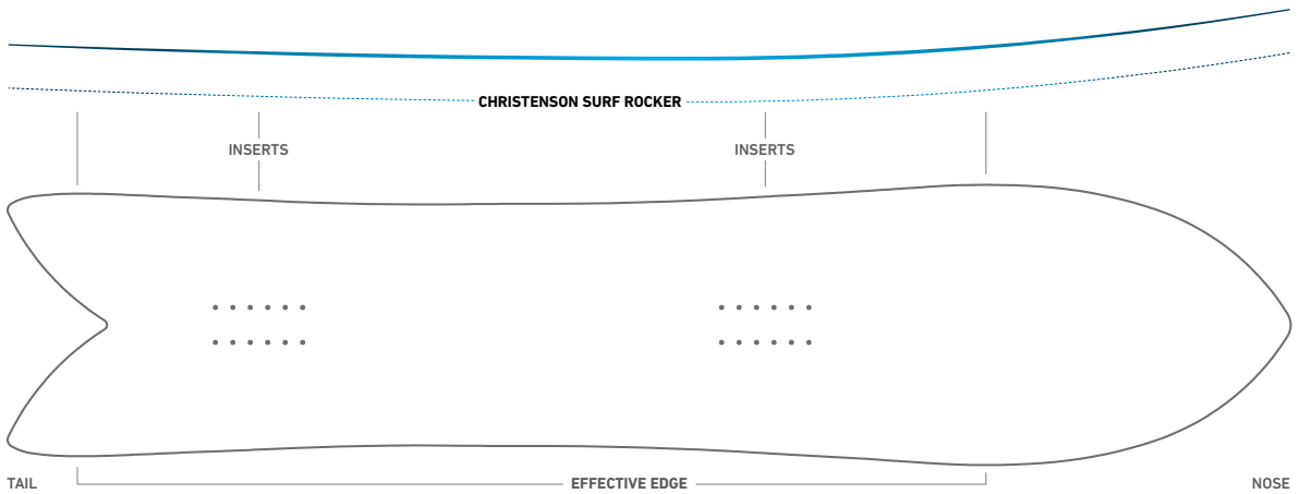
Drawing of the Storm Chaser, size 147
