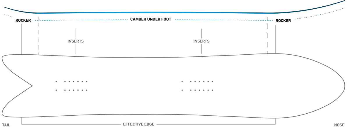
Drawing of the Storm Wolf, size 168
