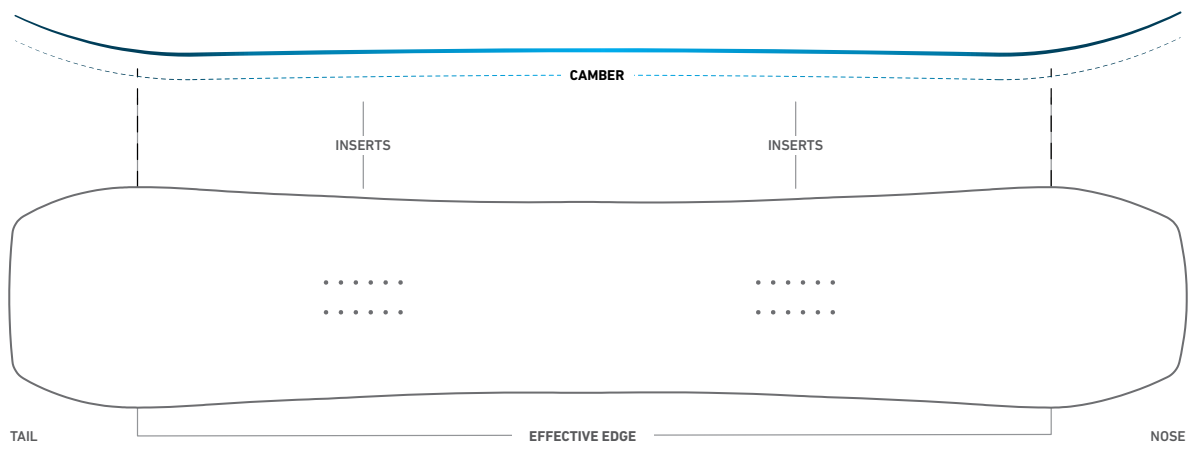
Drawing of the Aviator 2.0, size 158
