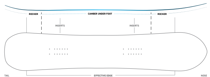
DRAWING OF THE MEN'S FRONTIER 2.0, SIZE 159
