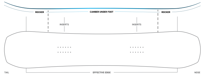
DRAWING OF THE MEN'S MOUNTAIN TWIN, SIZE 157
